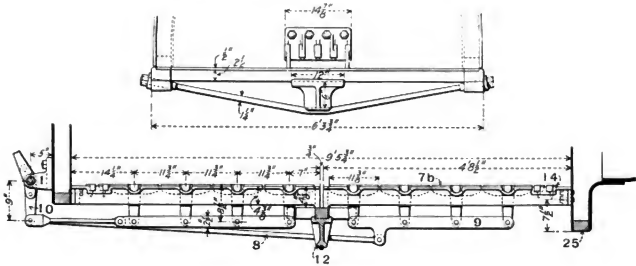
Fig. 521. Ashpan for Mogul (2-6-0) Locomotive. Pennsylvania Railroad.
